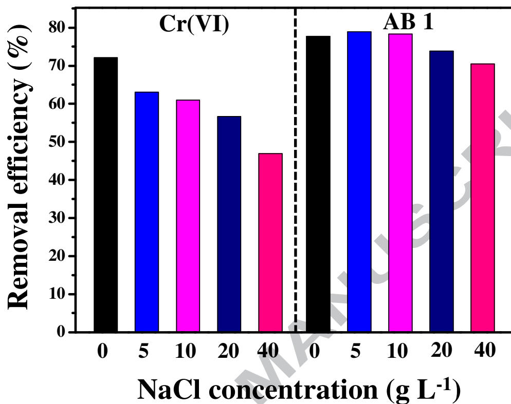
Fig. 13. Effect of ionic strength on the adsorption of Cr(VI) and AB 1 by prepared amino-functionalized SiO 2 @CoFe 2 O 4 -GO. (pH 2 for AB 1 and pH 1 for Cr(VI) ions, contact time: 140 min, temperature: 25°C, adsorbent dosage: 0.5 g L -1 , initial concentration: 10 mg L -1 )
