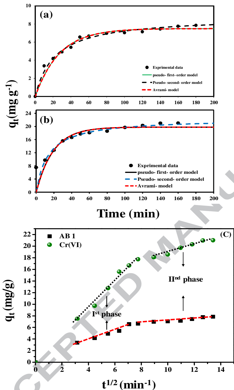
Fig. 11. Kinetic studies of (a) AB 1 and (b) Cr(VI) adsorption by amino-functionalized \text{SiO}_2@CoFe_2O_4 -GO nanocomposites, fitting of different kinetic models to the experimental data and Intra-particle diffusion model of AB 1 and Cr(VI) ions. (pH 1 for Cr(VI) ions and pH 2 for AB 1, adsorbent dosage: 0.5 \text{ g L}^{-1} , initial concentration: 10 \text{ mg L}^{-1} , temp: 25^\circ\text{C} )
