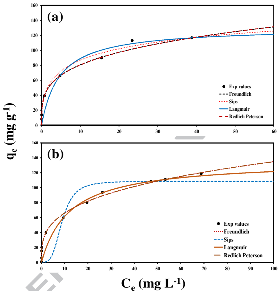
Fig. 12. Adsorption isotherms of (a) AB 1 and (b) Cr(VI) by amino-functionalized \text{SiO}_2@ \text{CoFe}_2\text{O}_4 -GO nanocomposites and fitting of different isotherm models to the experimental data. (Contact time: 140 min, pH 1 for Cr(VI) ions and pH 2 for AB 1, adsorbent dosage: 0.5 \text{ g L}^{-1} , temp: 25^\circ\text{C} )
