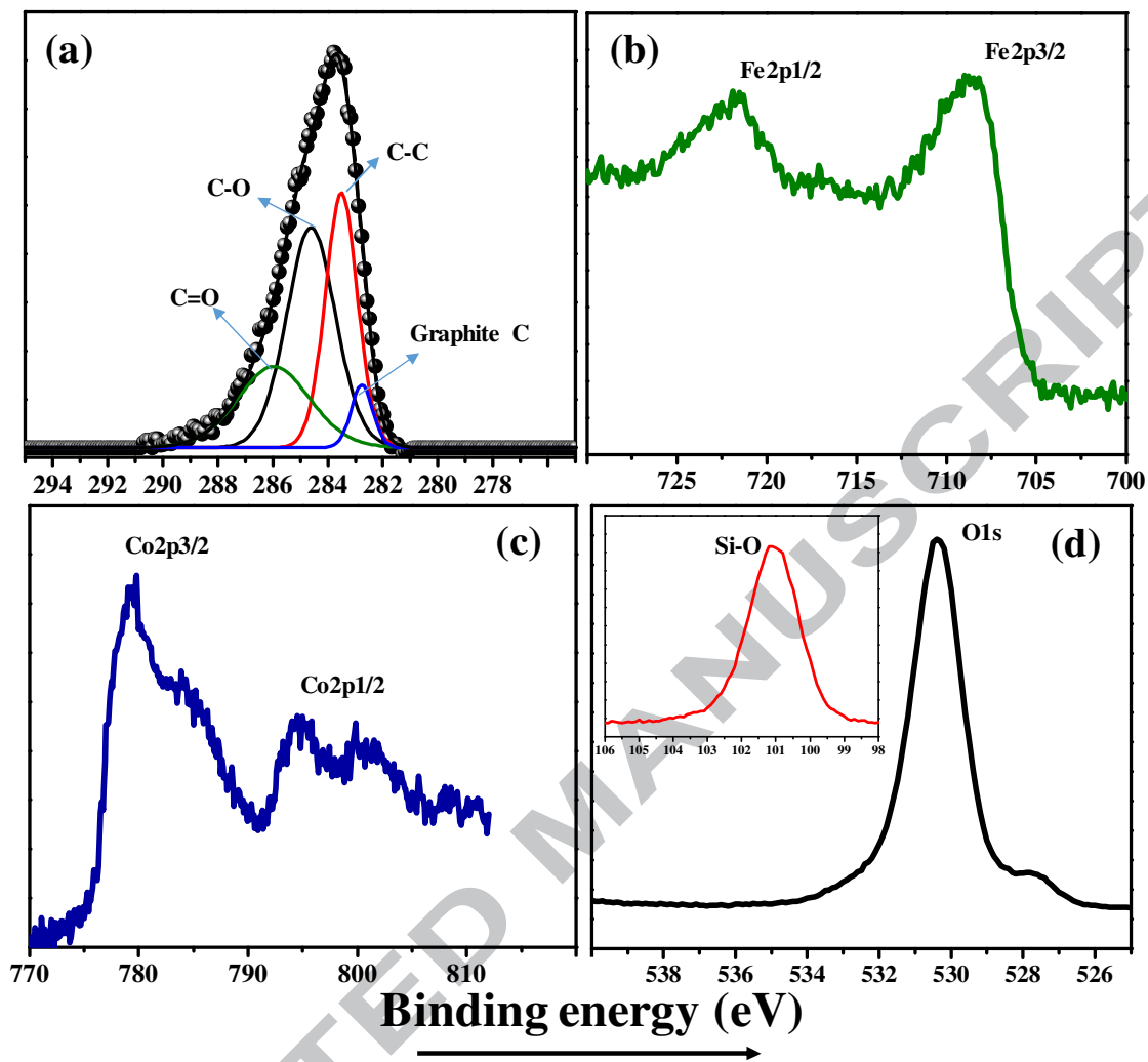
Fig. 8. XPS spectra of (a) C1s (b) Fe2p (c) Co2p and (d) O1s (Inset shows SiO 2 ) regions of amino-functionalized SiO 2 @CoFe 2 O 4 -GO nanocomposites.
