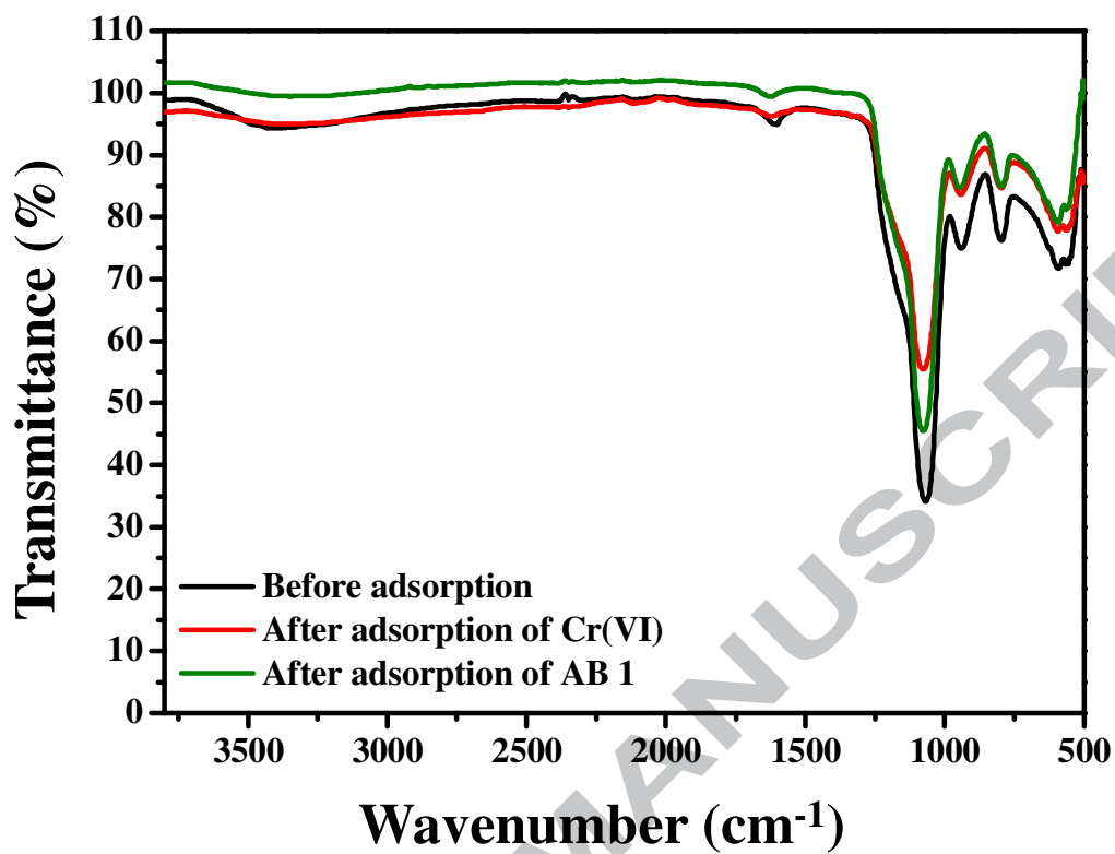
Fig. 15. FT-IR spectra of amino-functionalized SiO 2 @CoFe 2 O 4 -GO before and after adsorption of Cr(VI) and AB 1 ions.
