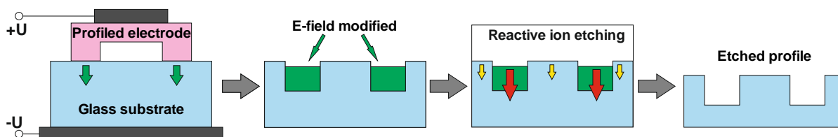
Figure 1. Schematics of thermal electric-field modification and reactive ion etching.
