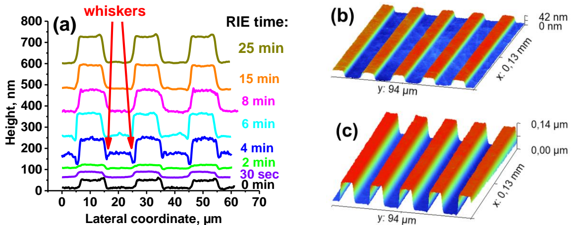
Figure 3. Reactive ion etching of the TEFI glass. Surface profile of RIE TEFI-processed 20 μm in period grating (a) and 3D plot of optical profiler data after the TEFI (b) and after the RIE (c). The glass was modified at 300°C under 300 V voltage; the TEFI with pressed glassy carbon electrode.
