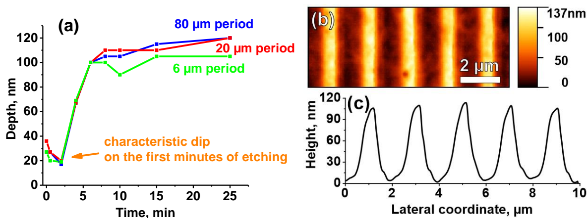
Figure 4. Depth of the gratings during the RIE process (a); AFM image (b) and surface profile (c) of 2 \mu\text{m} in period grating of glass RIE TEFI-modified at 300^\circ\text{C} under 300 V voltages. TEFI with pressed glassy carbon electrode.
