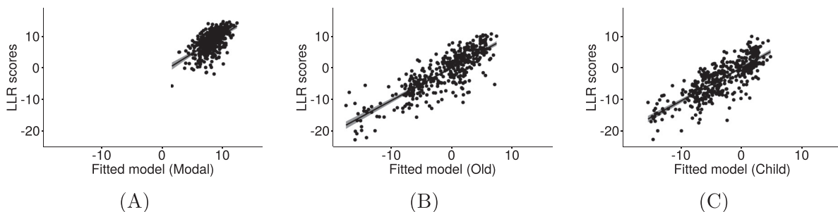
FIG. 5. Correlation for fitted model values and LLR scores (x-vector) for female speakers in their (A) modal ( r = 0.57 ), (B) intended old ( r = 0.83 ), and (C) intended child voices ( r = 0.80 ).
