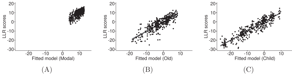
FIG. 6. Correlation for fitted model values and LLR scores (x-vector) for male speakers in their (A) modal ( r = 0.67 ), (B) intended old ( r = 0.82 ), and (C) intended child voices ( r = 0.92 ).
