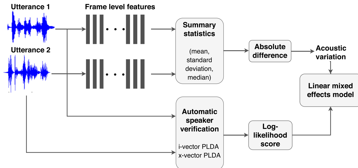
FIG. 1. (Color online) Procedure for the acoustical comparison of two utterances and assessment with LLR. The long term features are extracted from the trial utterances and then represented by summarized statistics. The features are compared and the absolute difference is estimated to represent the acoustic variation of the trial. This variation is then used to model the LLR score associated with the trial. ASV systems in this study include the i-vector and x-vector, both with PLDA scoring back-end.
