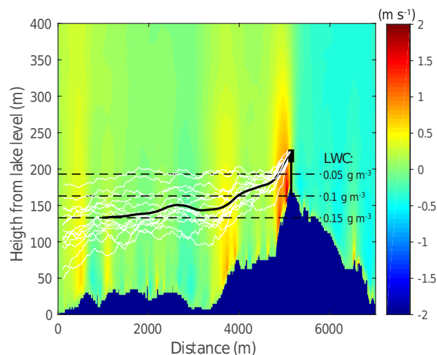
Figure 4. Simulated average wind fields and example trajectories (white curves) of air parcels. The black line depicts the average over all simulated trajectories.
