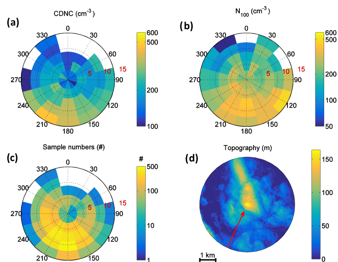
Figure 2. CCN dependence on wind speed and direction: (a) CDNC, (b) N_{100} , and (c) number of CDNC samples. (d) Topography of the area around Puijo hill, with the wind direction used in the simulations marked as red arrow.
