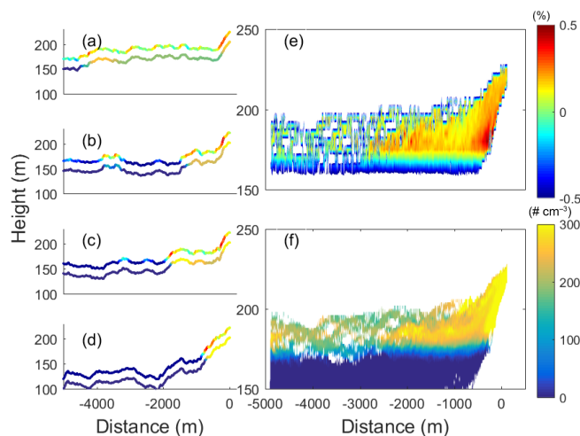
Figure 5. (a–d) Selected trajectories with supersaturation and CDNC superimposed. The two curves in each plot show the same trajectory, but are offset in y direction for easier distinction. The upper curve shows the correct height. (e) Average supersaturation over all simulated trajectories. (f) Average CDNC over all simulated trajectories.
