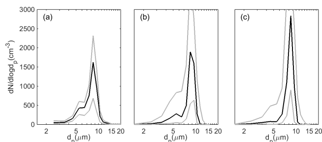
Figure 6. (a) Measured cloud droplet distribution. (b) Simulated cloud droplet size distributions using only trajectories that lead to second activation. (c) Simulated cloud droplet size distribution using all trajectories. Black lines denote the ensemble median, while grey lines denote the 10th and 90th percentile.
