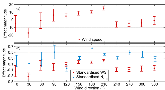
Figure 3. (a) Effect magnitude of wind speed on CDNC ( \partial\text{CDNC}/\partial v ) for different wind direction intervals and (b) standardised effect magnitude of wind speed and N_{100} on CDNC.
